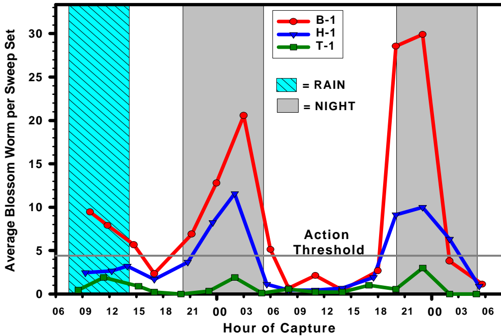
Figure 2. Same data as Figure 1, combined over the three sites to show frequency of all sweep captures in May 1999 for BLOSSOMWORM versus TIME of DAY
