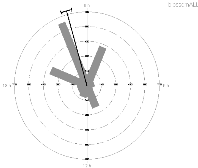
Figure 2. Same data as Figure 1, combined over the three sites to show frequency of all sweep captures in May 1999 for BLOSSOMWORM versus TIME of DAY
